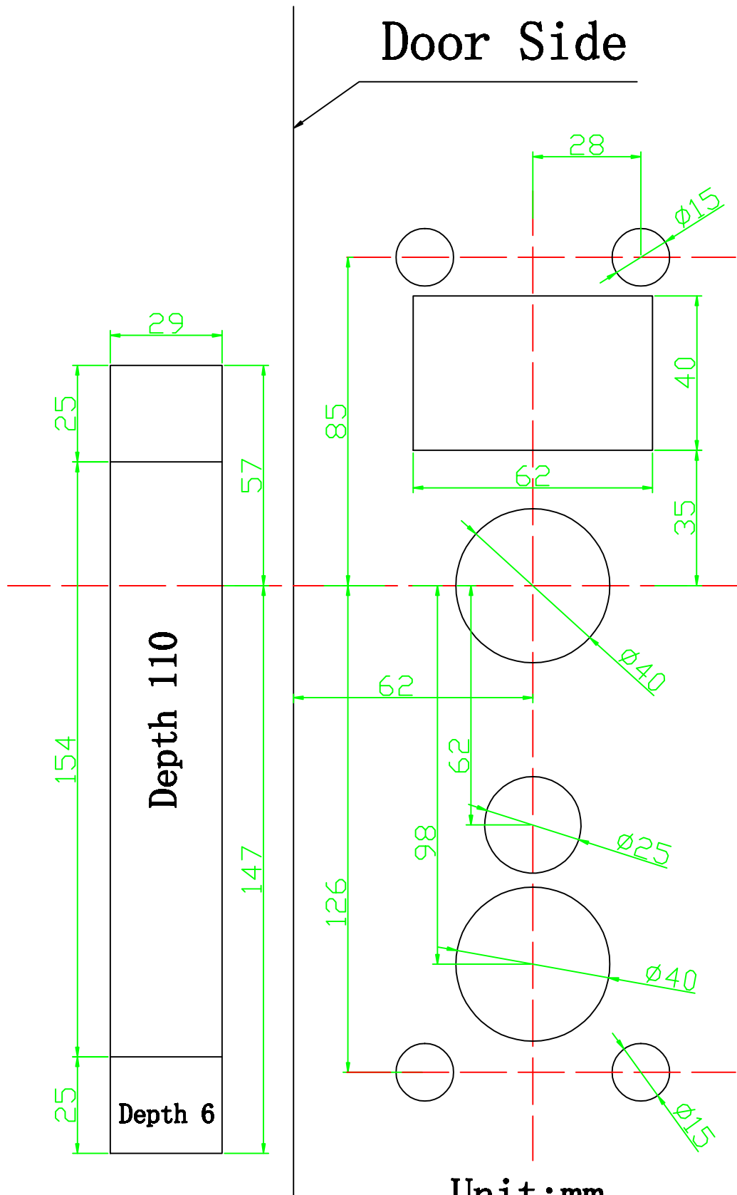
AR-S616-1 Hole Sketch
