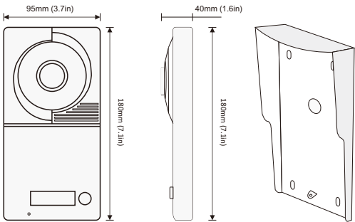
Rain cover
