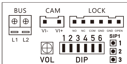
Connection Port
